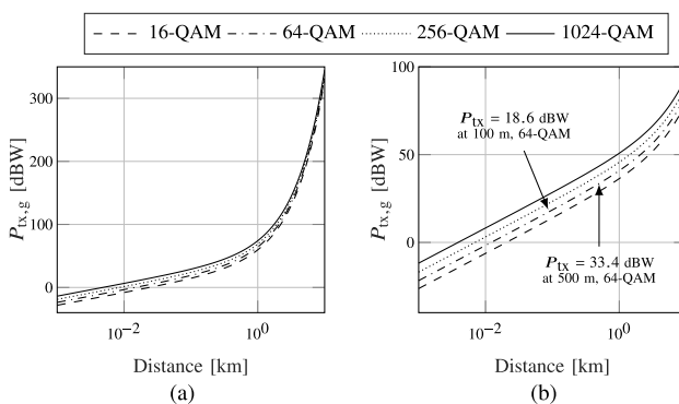
Fig. 9. Transmit power P_{\text{tx,g}} to achieve a 1-Tb/s data rate with a bit error rate smaller than 10^{-5} for different modulations and as a function of the distance between the terrestrial transmitter and receiver. (a) f_c = 183 GHz. (b) f_c = 230 GHz.
