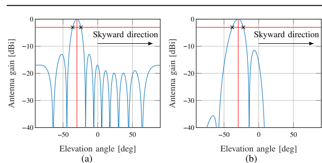
Fig. 13. Utilization of active suppression on the skyward directions during the array synthesis can suppress unwanted emissions. In both cases, the desired angle of steering is 30^\circ below the horizon. (a) Conventional beamforming. (b) Smart beamforming.
